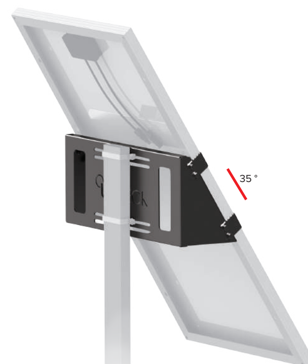
UNIFIX 100SF Pour Unisun 30.12M/50.12M/55.12BC/80.12M/100.12M/100.24M/110.12BC Orientation portrait Tête de mât Ref 1146
