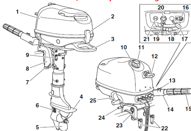
F5B,F6 Components Diagram
