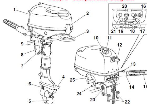
F5B,F6 Components Diagram
