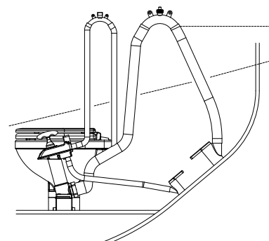
Fig. 1 Toilet below the waterline
